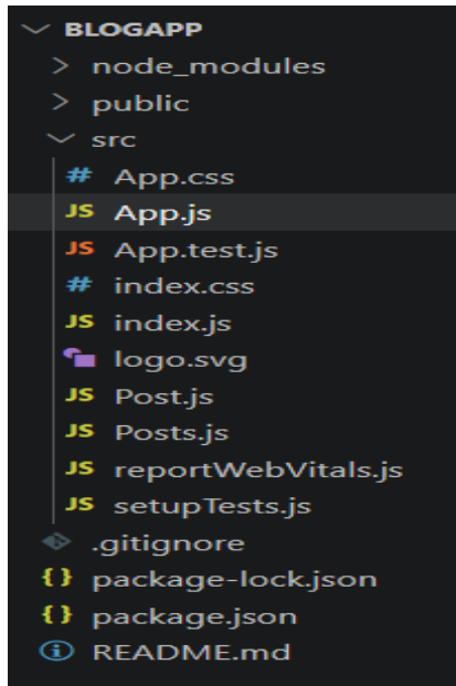
Figure 1: Project Structure
